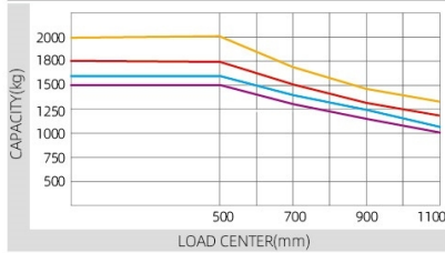
Load Curve
